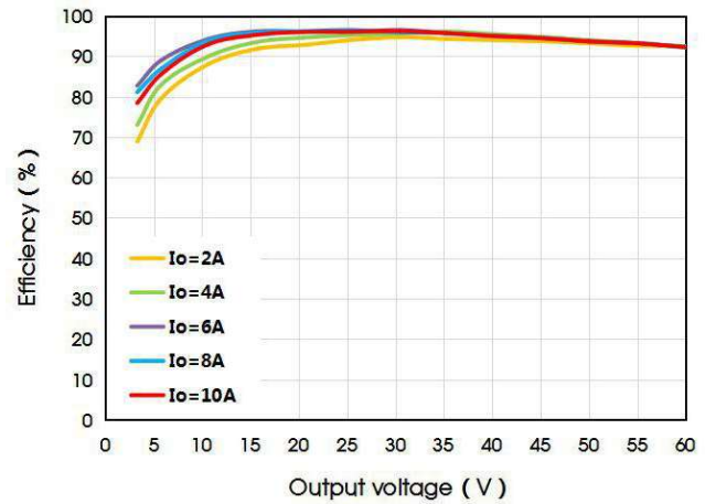
Efficiency VS Output voltage (Vin=60V)
