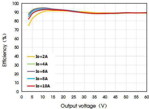
Efficiency VS Output voltage (Vin=48V)
