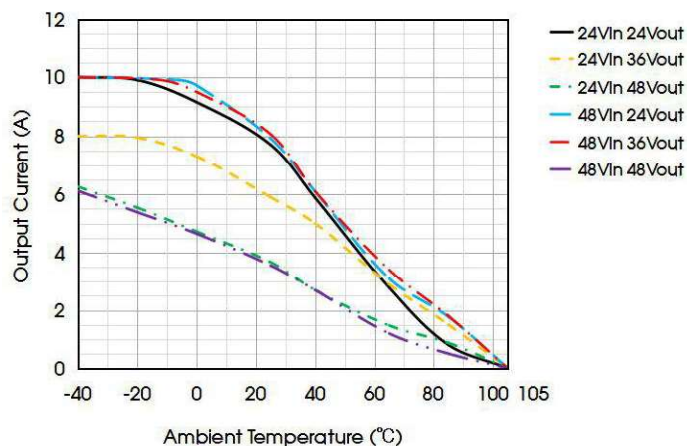
SKUB4836EB-10A (-RS) Temperature Derating Curves (20LFM)
